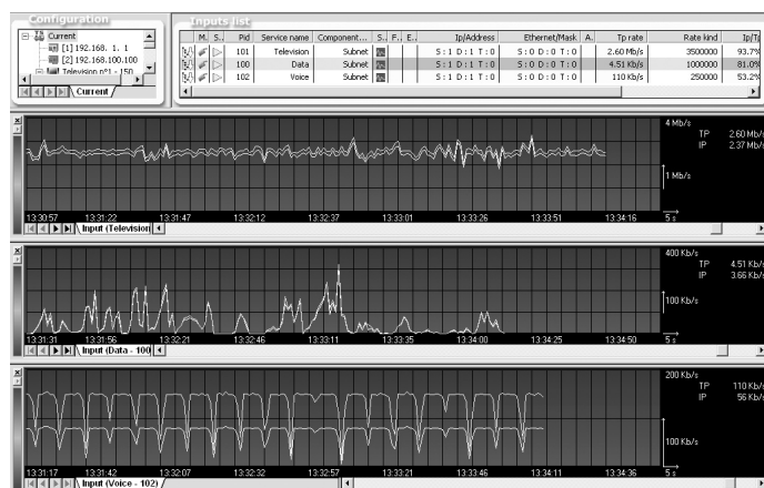
Fig.2. The satellite triple play multiplex, as monitored in the DVB-S2 Multiplexer; per-service traffic view (video, data, voice).
