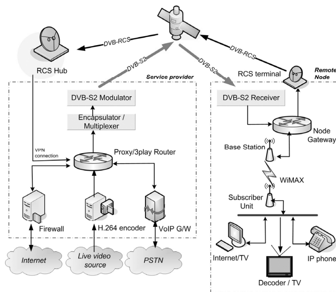
Fig. 1. The developed satellite infrastructure for triple play services
