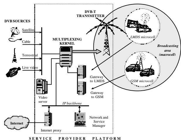
Figure 1: General System Configuration
