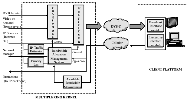
Figure 2: The bandwidth optimisation mechanism
