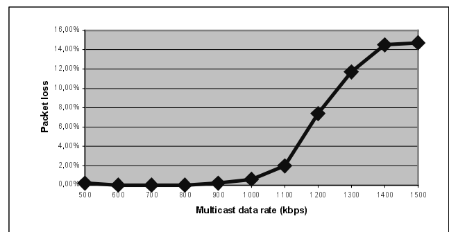
Fig. 5 Data packet loss vs. multicast rate
