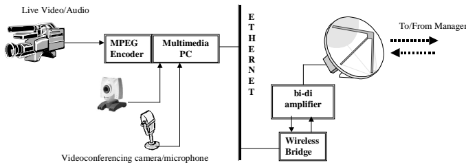
Figure 2: Agent structure
