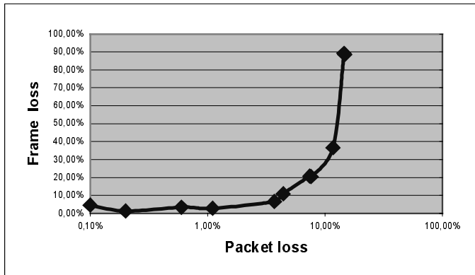
Fig. 6 Video frame loss vs. data packet loss in the MPEG stream
