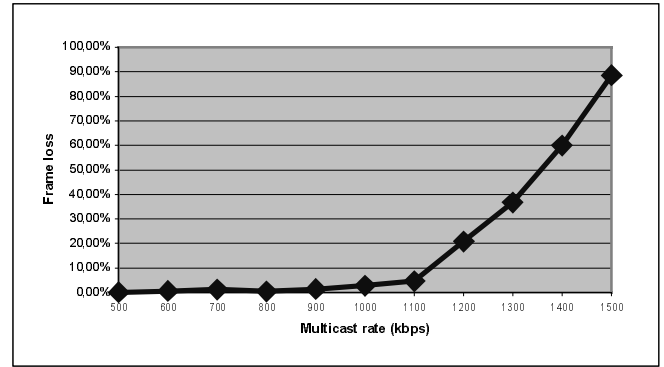
Fig. 7 Video frame loss vs. Multicast rate
