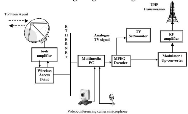
Fig. 3 Manager structure
