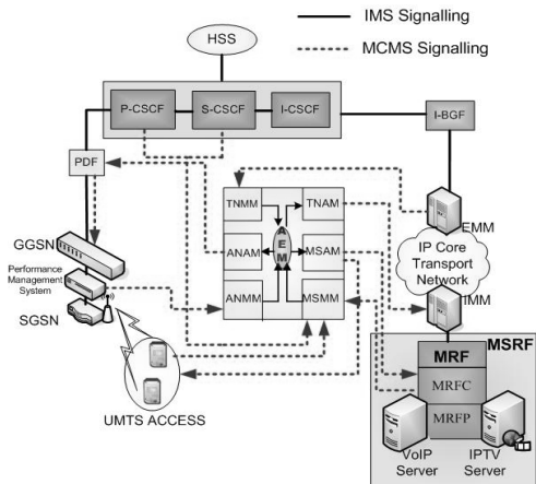
Figure 2. The ADAMANTIUM MCMS and NGN IMS architecture
