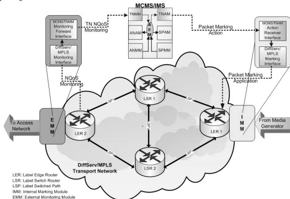
Figure 4. ADAMANTIUM DiffServ/MPLS Core Network Architecture
