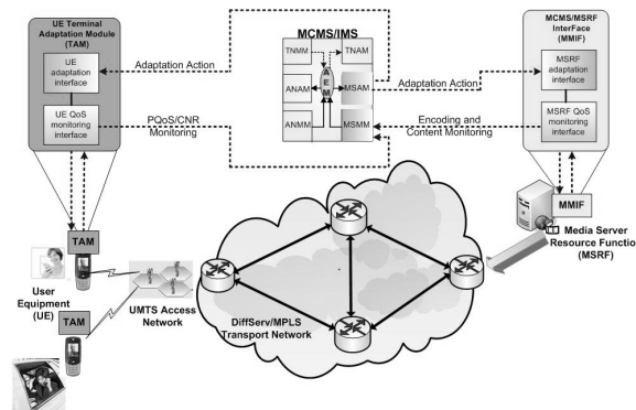
Figure 5. The Modules Interaction for IPTV Service Adaptation
