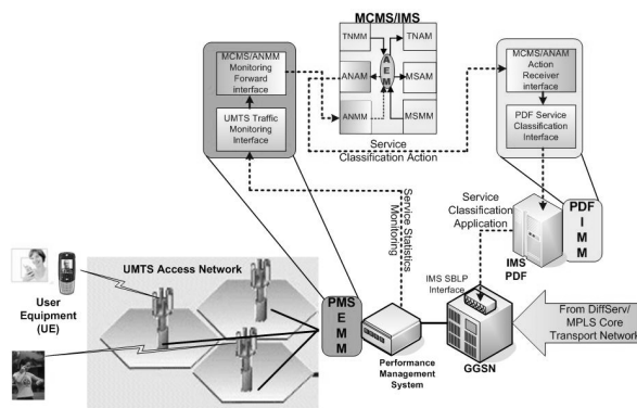
Figure 3. The ADAMANTIUM Access Network Architecture
